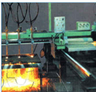
Photoelectric Tracing Cutter
